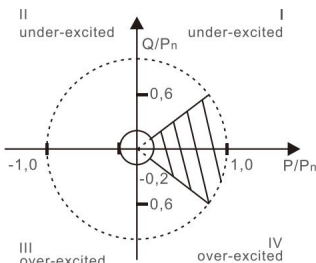
Figure 6.24 Plage PF
